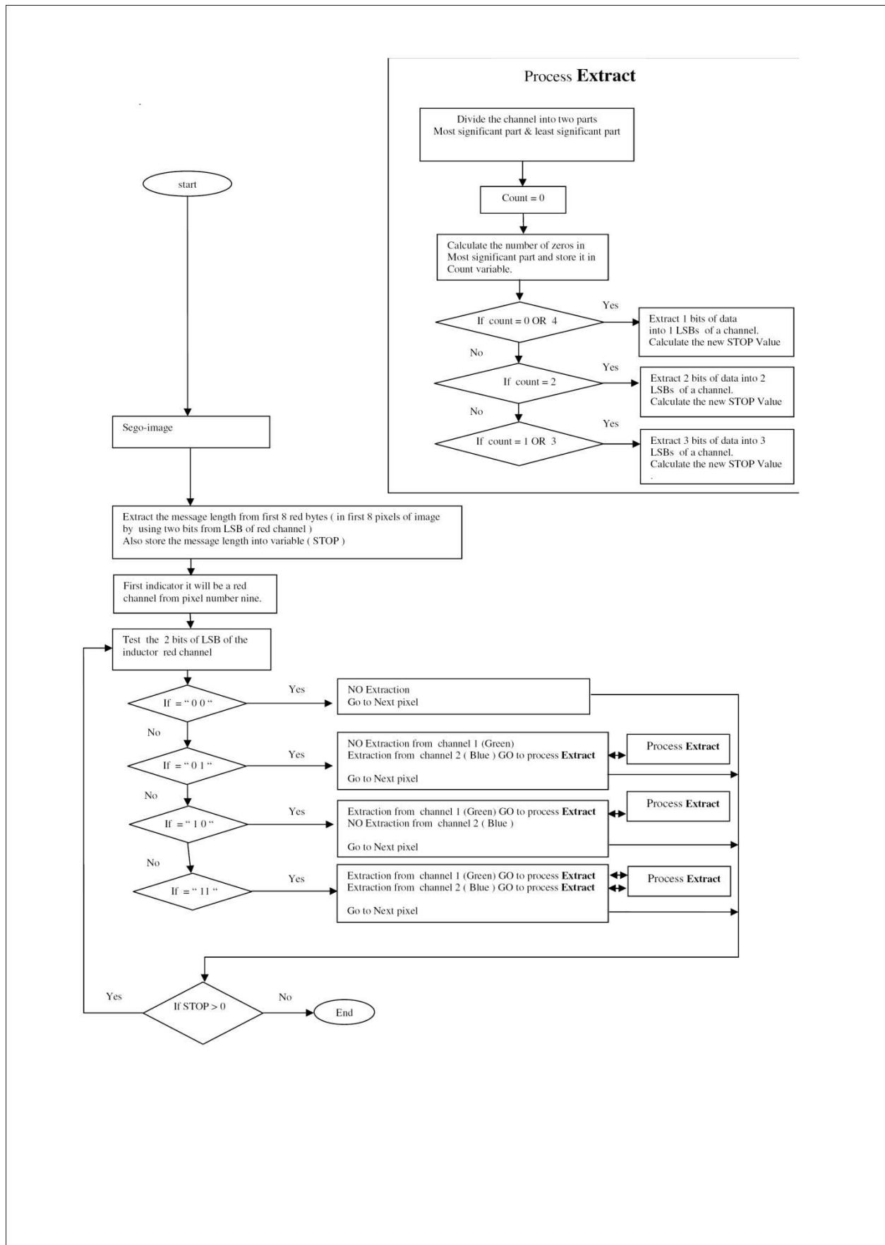
Figure (0-7) Flowchart of a proposed extraction algorithm
