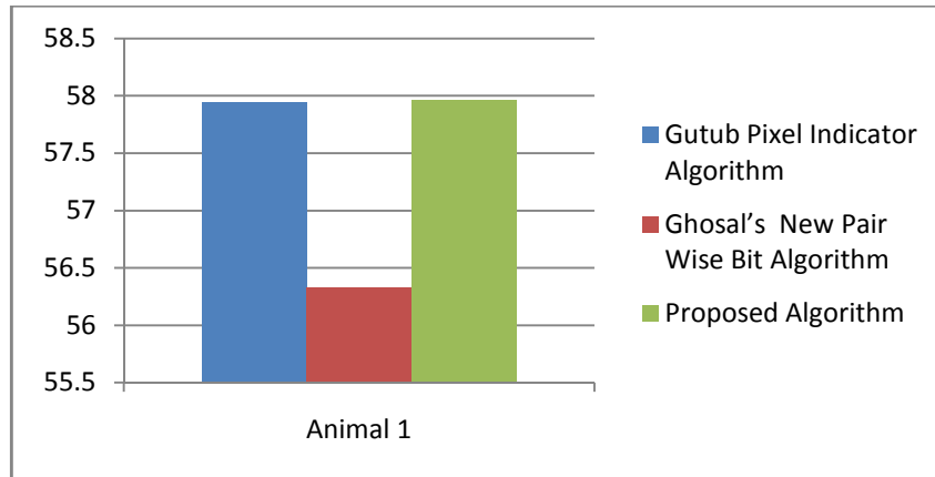
Figure (0-8) Shows the PSNR test for Animal 1 image
