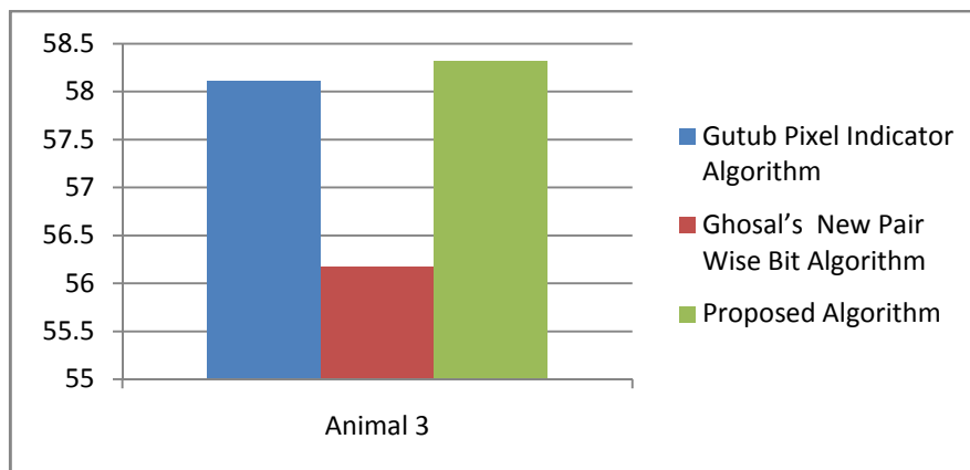
Figure (0-10) Shows the PSNR test for Animal 3 image
